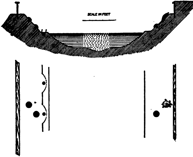
FIG. 2. — Section and plan of a turtle-pond
